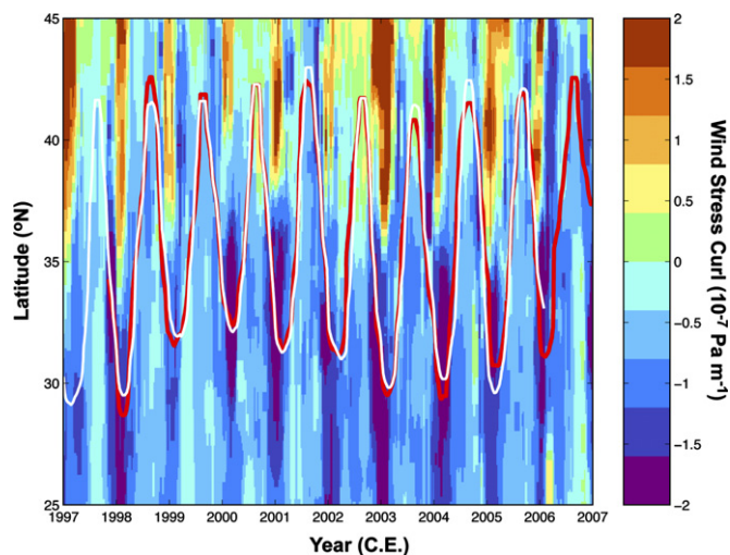
Fig. 2. Time series of Chla and SST fronts, defined by the 0.2 mg m -3 isopleth (red line) and the 18 °C isotherm (white line), respectively. The background is wind stress curl (negative indicates convergence).
